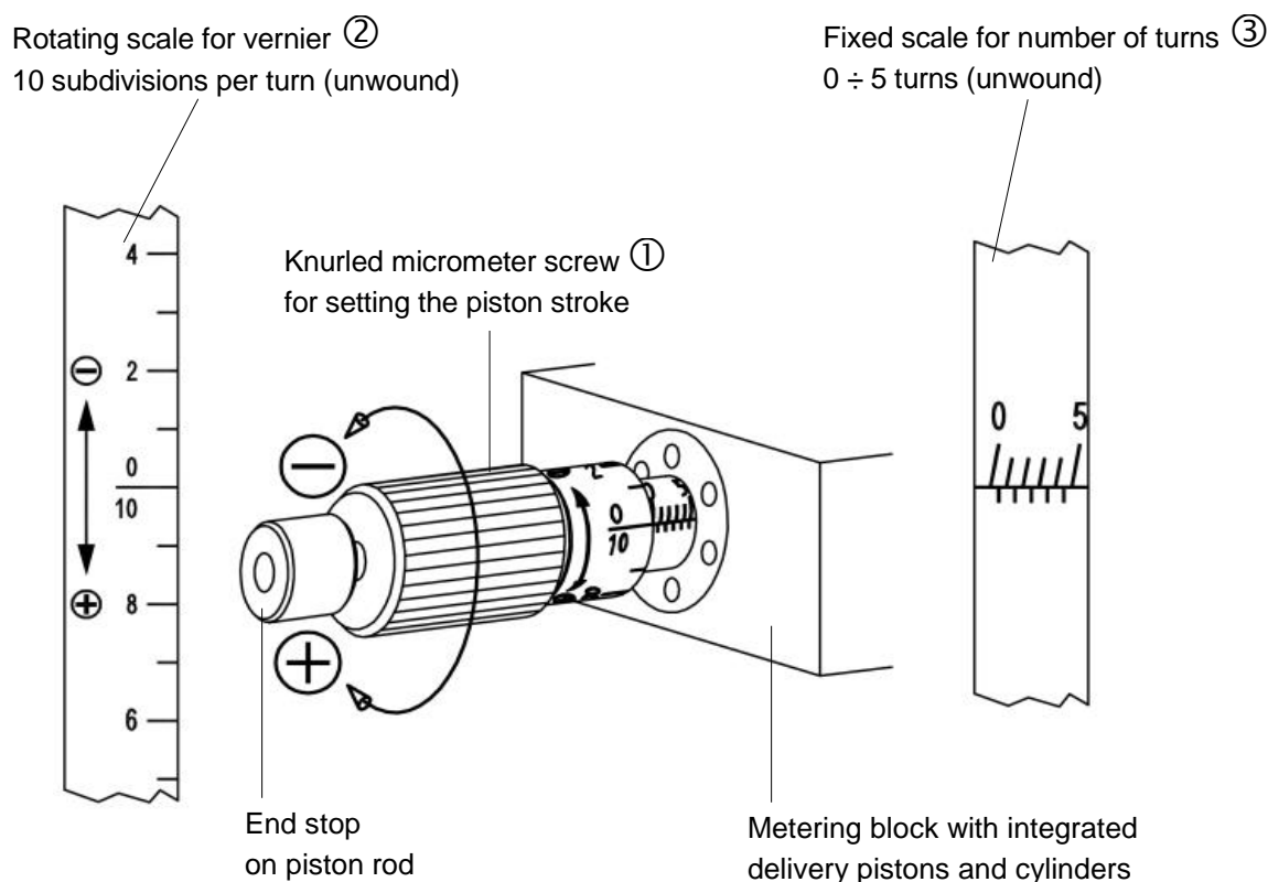
Fig. 11: Metering pump – regulating knob, metering stroke setting with micrometer display for stepless adjustment 0 ÷ 5 turns (10 ÷ 100% delivery rate)
