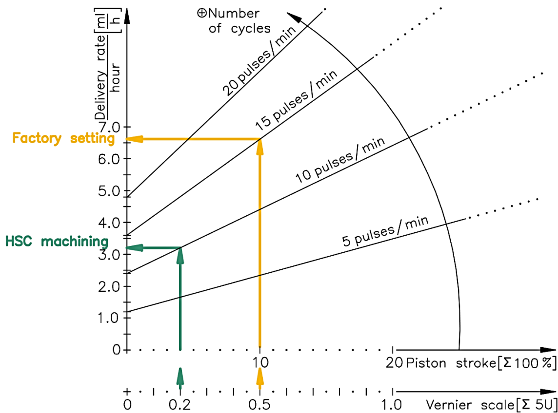
Fig. 21: Consumption as a function of the piston stroke and at different cycle rates (pulses/min)
