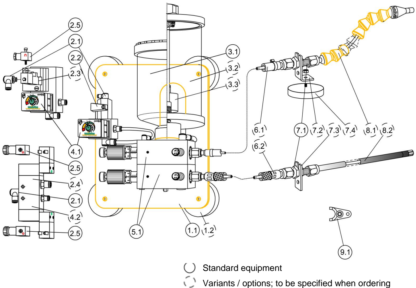
Fig. 2: POPLUBE Minimal Lubrication System
