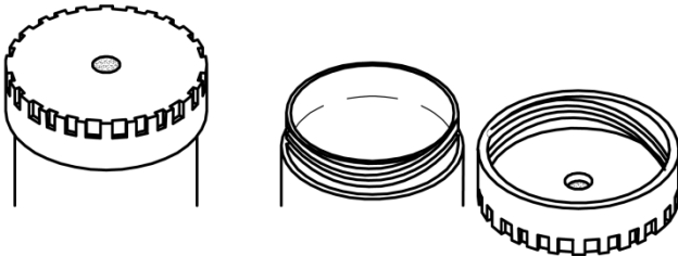
Fig. 9: 0.3 litre reservoir with screw cap
