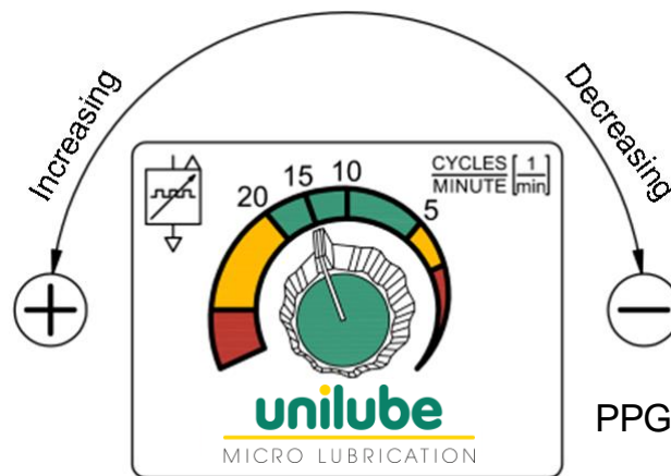
Fig. 12: Pneumatic Pulse Generator – setting number of cycles (5 ÷ 20 pulses/min)
